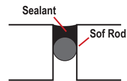
Sof Rod™ in expansion joints and similar applications
