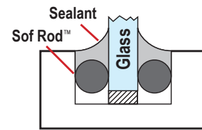
Sof Rod™ for Glazing
